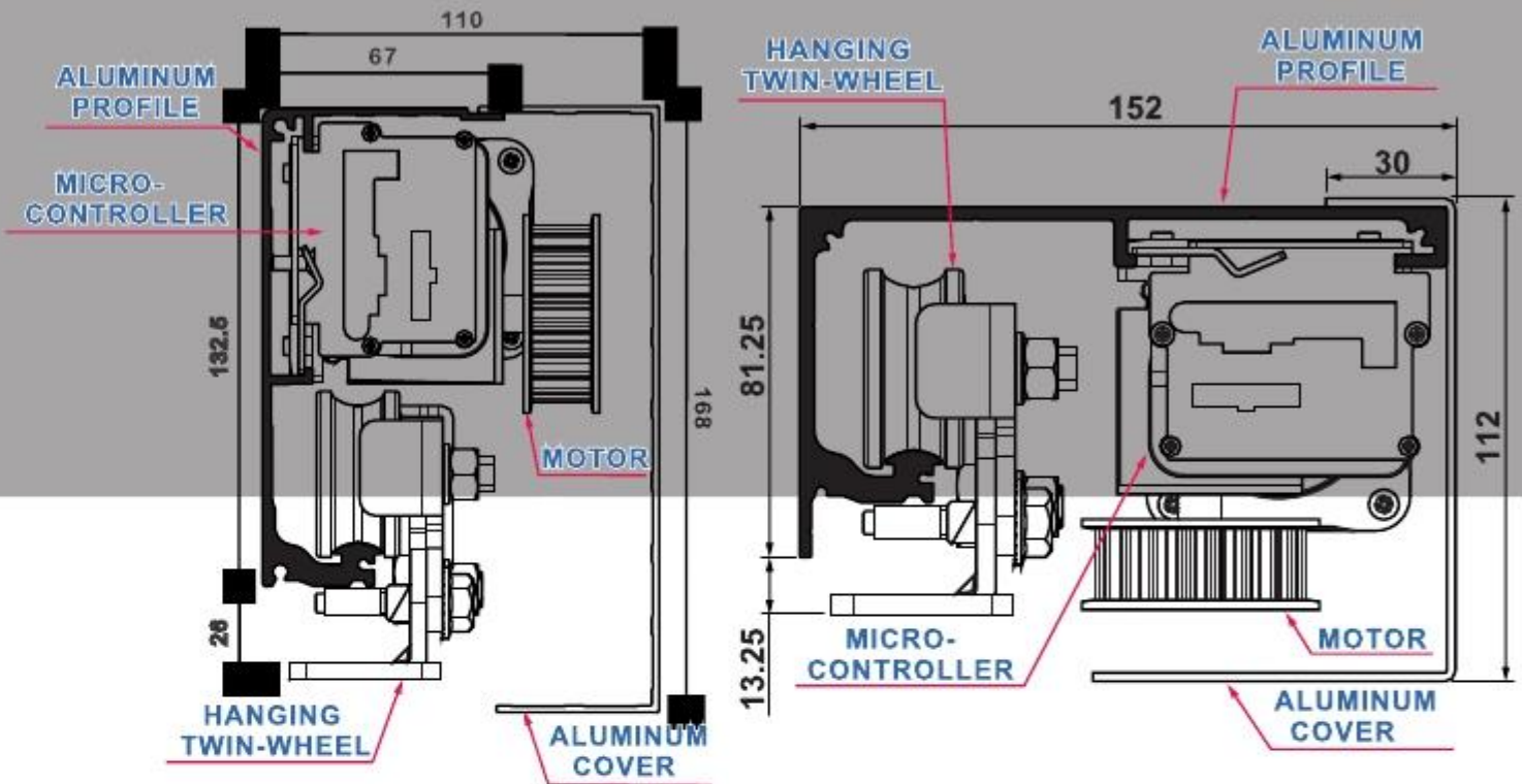
SECTIONAL DRAWING
